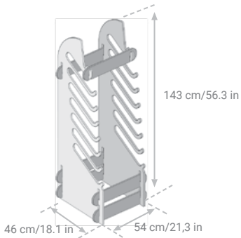
WOODEN STAND FOR 35 TUBES
